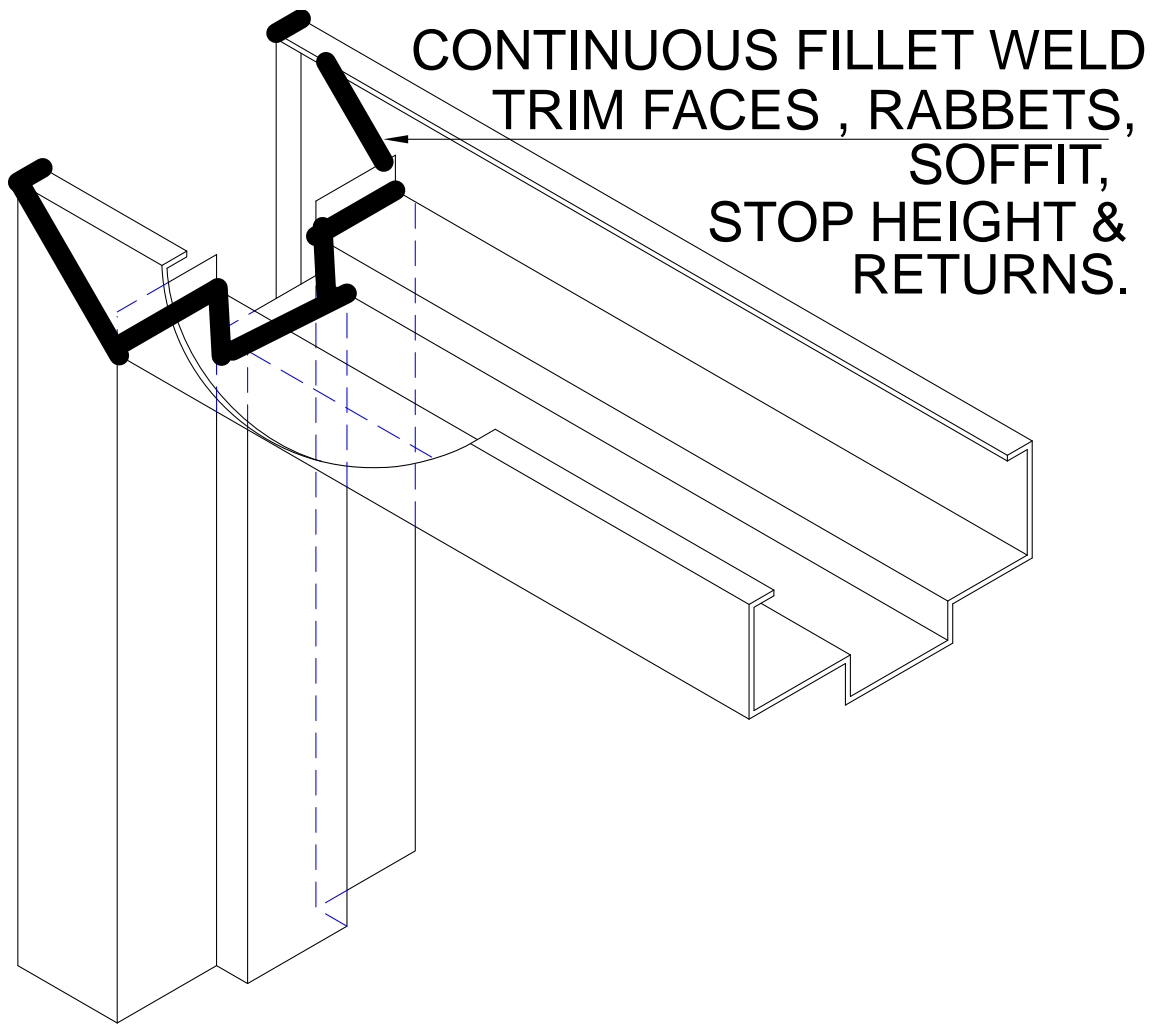
WELDED CORNER SECTIONS TYPE 2
