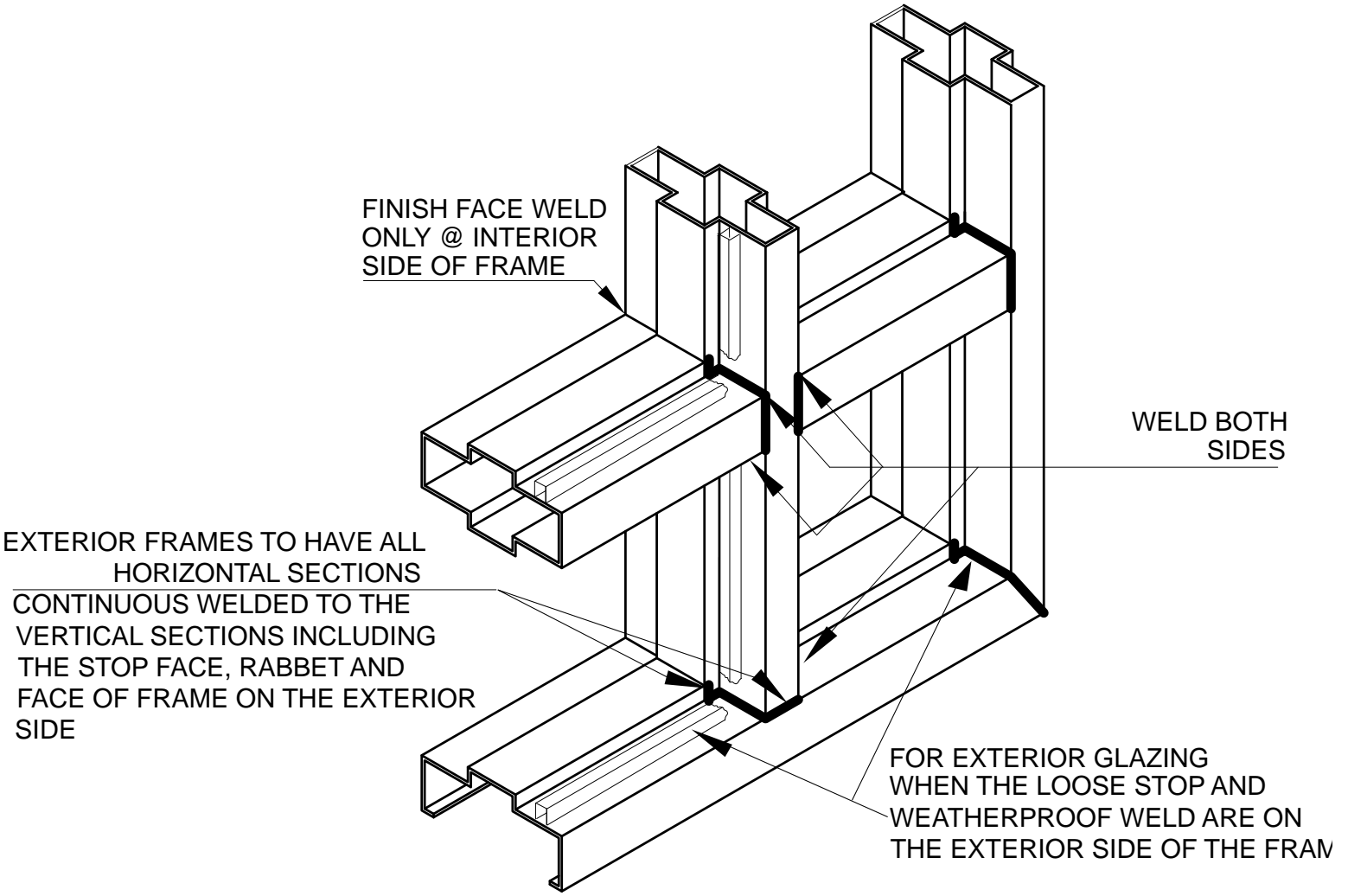
TYPE B FULL WELDED EXTERIORS ONLY.
