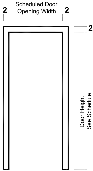
TYPICAL ELEVATION
