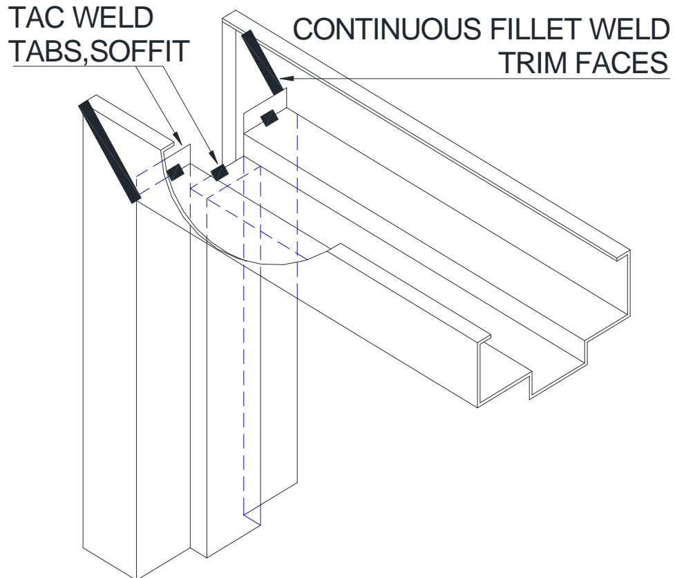
STANDARD WELDED CORNER SECTIONS TYPE 1
