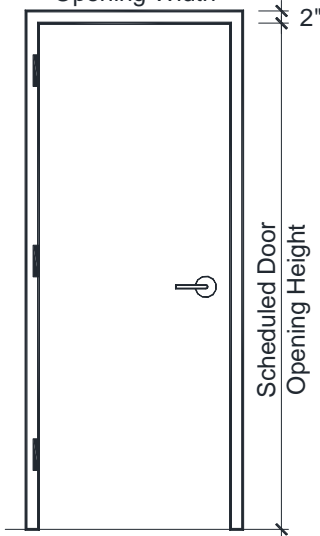
TYPICAL ELEVATION 2" Scheduled Door 2" Opening Width
